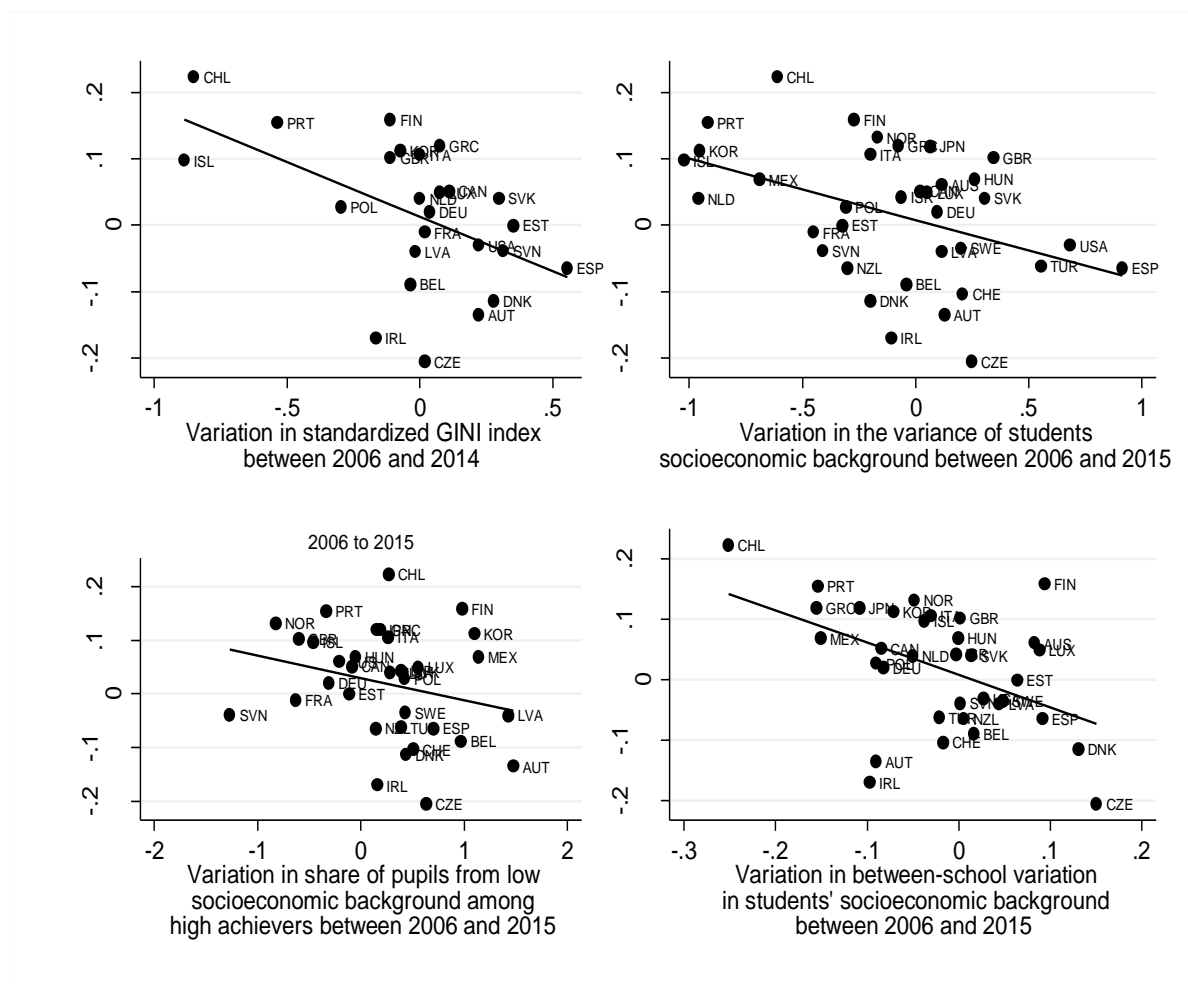
Figure S2: Country-level relationship between variations in four measures of inequalities and variations in the gender performance gap in math between 2006 and 2015.
