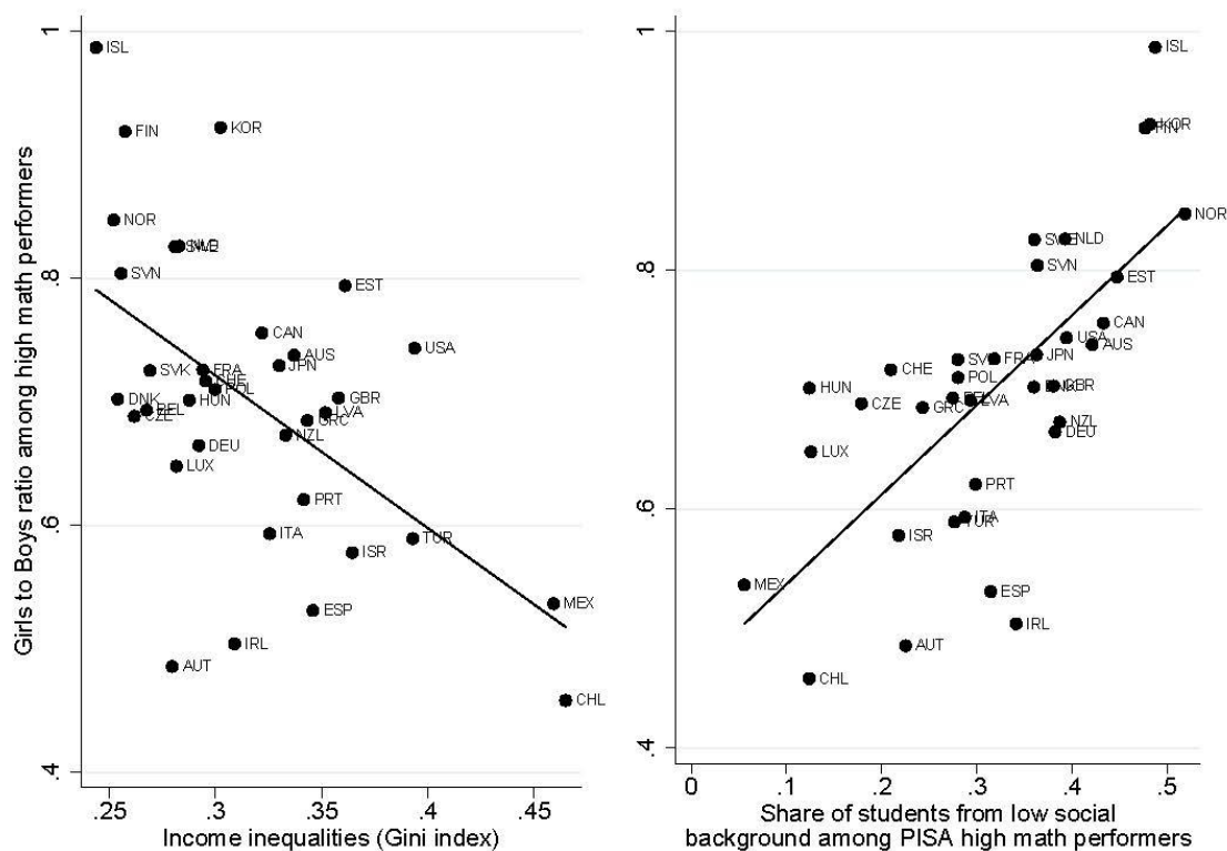
Figure S1: Two measures of Inequalities and Girls underrepresentation among high performers in mathematics among OECD countries
